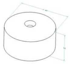
HPPA-HB-5904 Interchangeable Seat H02-100-64-0110D
