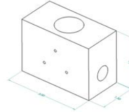
HPPA-00-OCT3 *Standard Combo 3/8" x 3/8" x 9/16" Tee Cross# H04-025-40-03018
