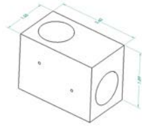
HPPA-00-00E9 Standard 9/16" Elbow Cross to H04-025-40-02002
