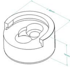
HPPA-HB-5808 Check Valve Cap D20-44-30-2006C
