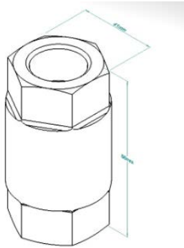
HPPA-HB-5701 Inline Check Valve Body H04-025-40-08017
