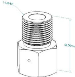
HPPA-HB-5701-2 Inline Check Valve Body Nut H04-025-40-08011*
