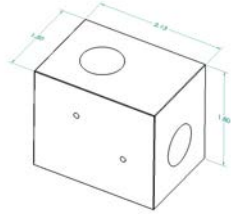
HPPA-00-00E3 Standard 3/8" Elbow
