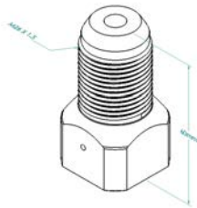
HPPA-HB-5805 Check Valve Outlet Poppet H02-250-60-0090Cv1
