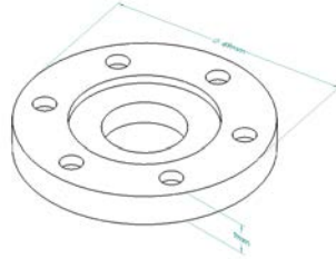
HPPA-HB-5806 Hydraulic Seal Cap D20-050-10-0003C
