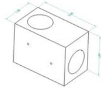
HPPA-00-00E9 Standard 9/16" Elbow
