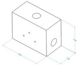
HPPA-00-00T3 Standard 3/8" Tee
